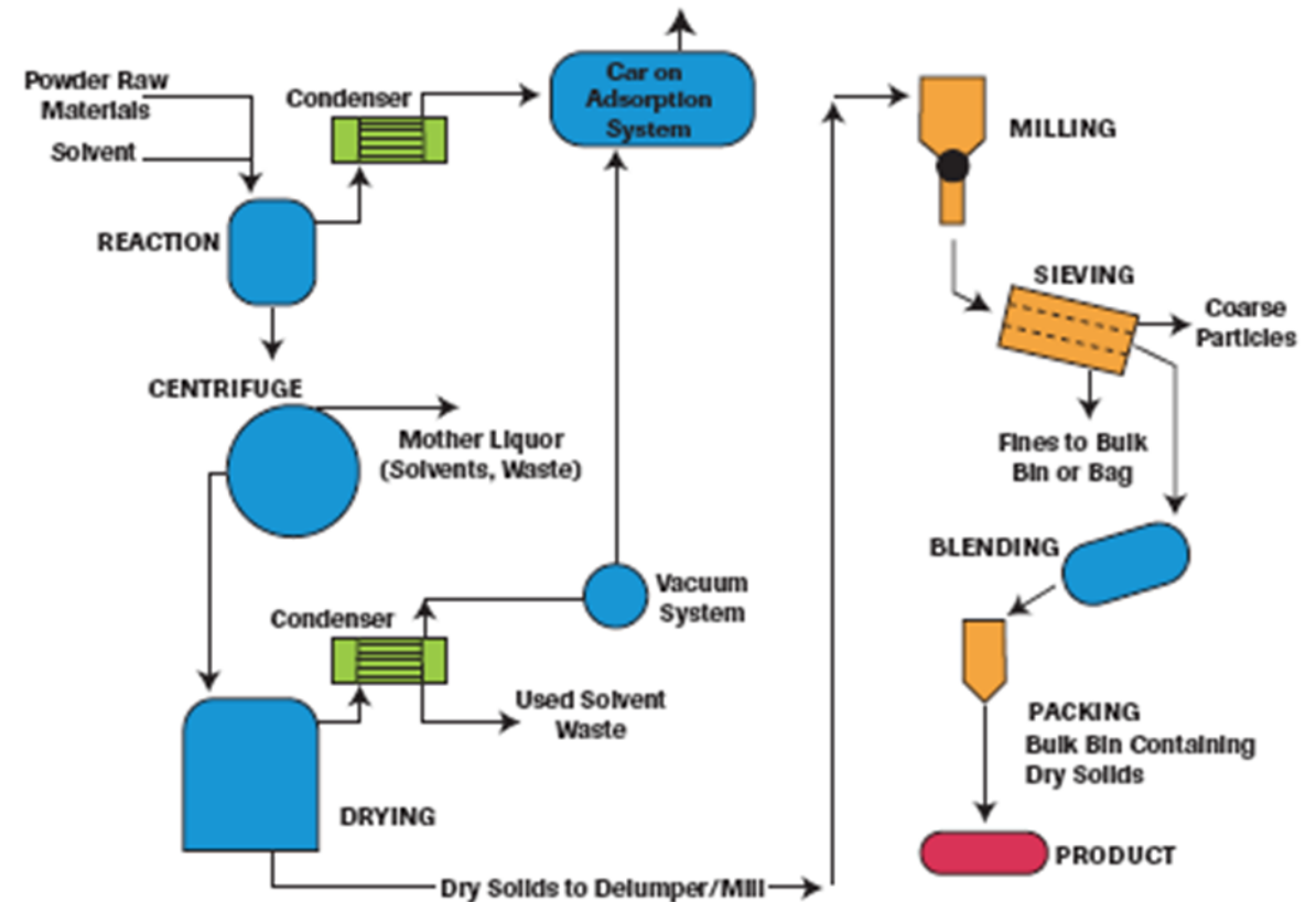
Generic Synthesis Route
